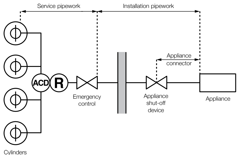
Figure 7(a) LPG systems – cylinder installation
