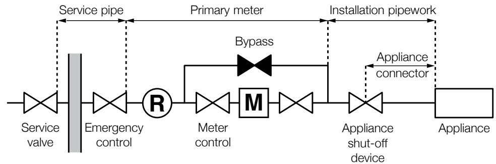
Figure 5 Meter with bypass, eg industrial/commercial
